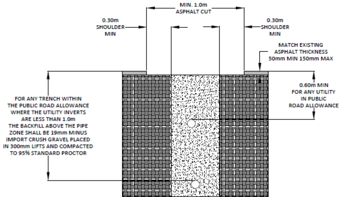
TYPICAL SECTION SCALE 1:25
