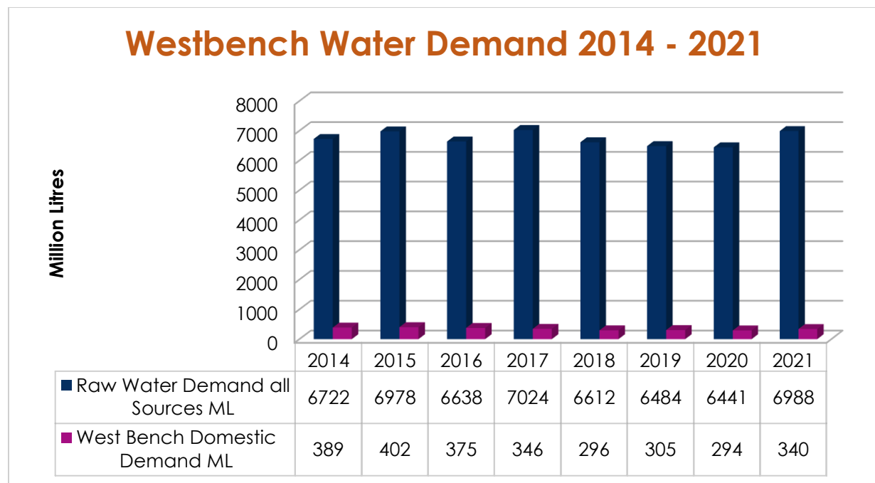
Chart 9: 2014 – 2021 Raw Water Demand / Including West Bench Irrigation District
