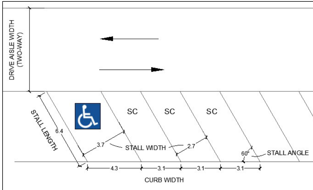
Figure 13 - Stall Size
