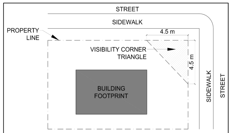
Figure 9 - Corner Visibility Triangle Diagram
